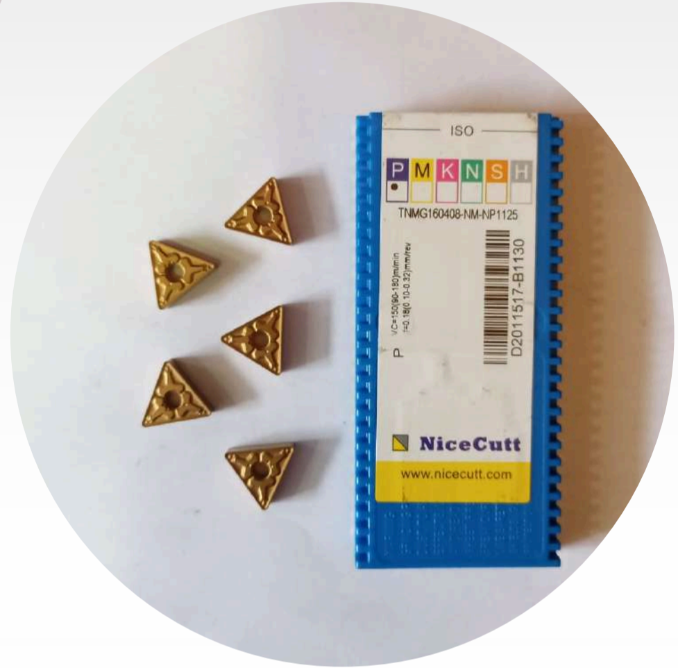
TNMG160408
