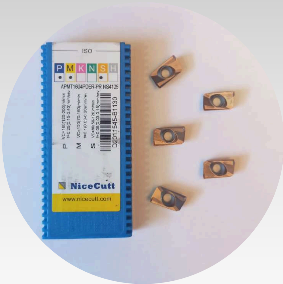
APMT1604PDER
